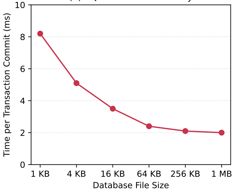
(a) SQLite Commit Latency
