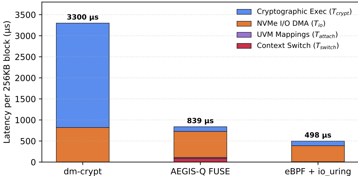
Write Latency Breakdown: CPU baseline vs. FUSE vs. eBPF+io_uring
