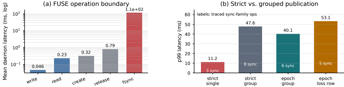
Figure 7: Graph-driven RQ5 cost boundary. Panel (a) shows daemon-side FUSE operation latency from retained traces; fsync dominates ordinary read/write/create costs. Panel (b) separates strict single-client publication from grouped epoch behavior: grouping can reduce traced sync-family operations, but the loss row shows why it is an admission rule rather than a replacement for strict publication.
