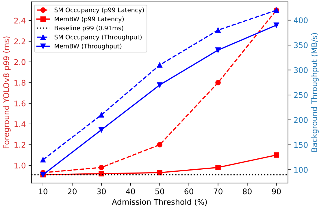
Asymmetry Ablation: SM Occupancy vs Memory Bandwidth
