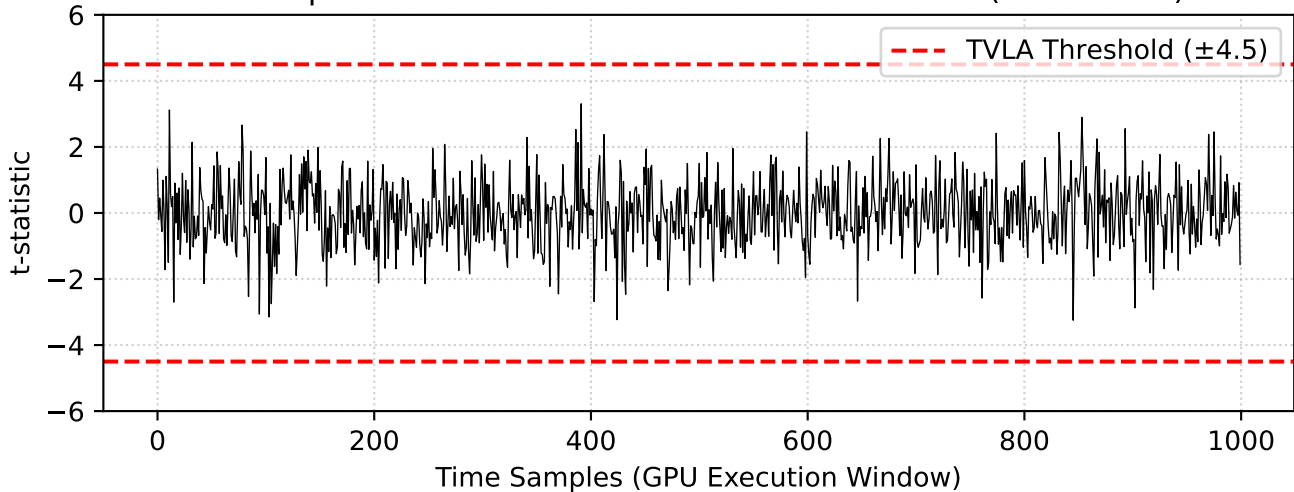
Non-Specific TVLA t-test for ML-KEM GPU Kernel (N=100000)
