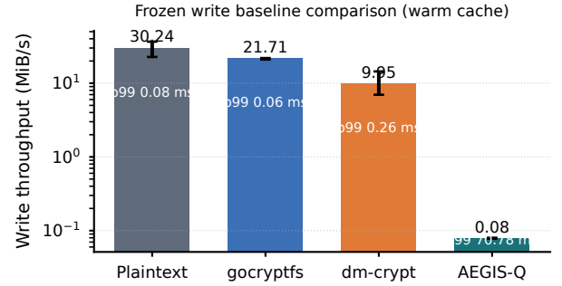
Figure 1: Frozen-contract write comparison for the baseline set (warm cache, 4 KiB randrw 70/30 with fdatasync). Bars report median throughput with 95% CI; labels report p99 latency.
