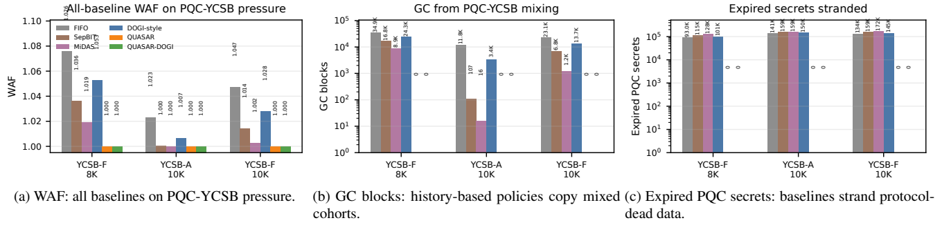
Figure 3: PQC lifecycle pressure on YCSB carriers, comparing all same-path baselines. The carrier supplies DOGI-friendly update locality; the side writes supply PQC objects whose invalidation follows protocol state. QUASAR and the hybrid keep payload on history placement and route PQC objects by death cohort, eliminating stale-secret exposure while reducing WAF/GC on pressure rows.
