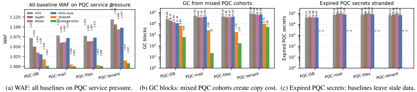
Figure 4: PQC lifecycle pressure breadth, comparing all same-path baselines. The x-axis names the service carrier, but the measured failure is PQC-specific: expired secret cohorts remain mixed with live payload under history-based placement. QUASAR and QUASAR-DOGI keep those cohorts reset-eligible while preserving payload placement on the history fallback.
