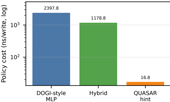
Policy decision cost
