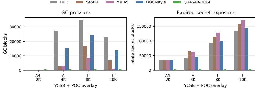
Figure 1: Actual-ZNS YCSB pressure with all history-based baselines. The low-pressure row is intentionally a negative WAF control, while higher PQC overlays create GC pressure. FIFO, SepBIT-style, MiDAS-style, and DOGI-style placement all leave expired secret blocks because they cannot see protocol death cohorts; QUASAR-DOGI keeps secret cohorts reset-eligible and removes the exposure on the same rows.
