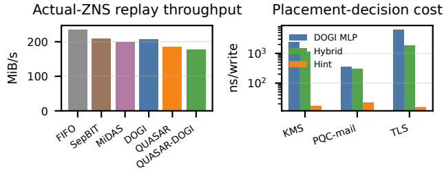
Figure 8: Prototype overhead in the role of DOGI’s prototype figure. Zonefs replay is an accounting bound, while the isolated C-level benchmark shows lifecycle-hint routing is much cheaper than DOGI-style feature extraction and MLP scoring.
