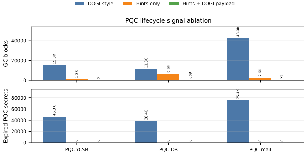
Figure 5: PQC lifecycle-signal ablation. A history-only DOGI-style policy sees storage history but misses cryptographic death cohorts, so GC and expired-secret exposure remain. Lifecycle hints remove exposure; adding DOGI-style payload fallback recovers payload placement and removes the remaining GC in the default hybrid.
