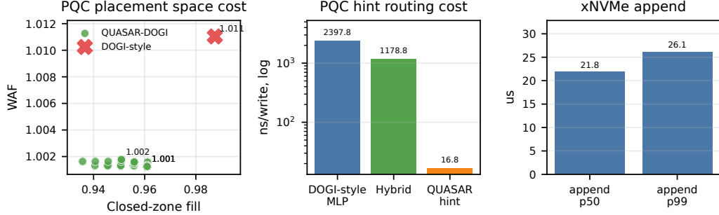
Figure 6: PQC placement resource and overhead controls. QUASAR-DOGI bounds the closed-zone fill cost while removing stale PQC secrets, the lifecycle-hint routing path is orders of magnitude cheaper than the DOGI-style policy-decision microbenchmark, and xNVMe confirms a lower-overhead append command path than the zonefs helper used for full-suite replay accounting.
