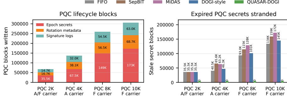
Figure 1: PQC lifecycle pressure on actual ZNS. The left panel shows the PQC artifacts that create the storage problem: epoch secrets, rotation metadata, and append-only signatures. The right panel shows the consequence after epoch close: FIFO, SepBIT-style, MiDAS-style, and DOGI-style placement strand expired PQC secret blocks, while QUASAR-DOGI keeps those death cohorts reset-eligible.
