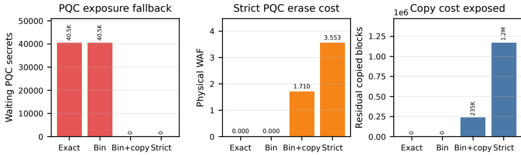
Figure 7: PQC robustness frontier. Exact and binned placement can leave delayed-expiry PQC secrets waiting under tight active-zone budgets. Residual migration removes the exposure but increases physical WAF and copied blocks; strict zero-wait mode is therefore a policy point, not the default.
