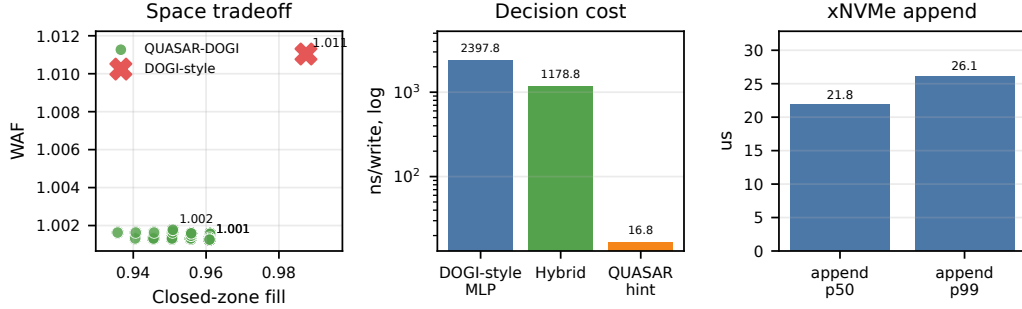
Figure 6: Resource and overhead controls. QUASAR-DOGI bounds the closed-zone fill cost while removing stale secrets, the hint-routing decision path is orders of magnitude cheaper than the DOGI-style policy-decision microbenchmark, and xNVMe confirms a lower-overhead append command path than the zonefs helper used for full-suite replay accounting.
