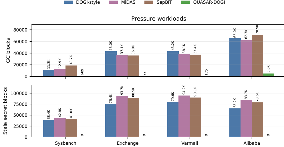
Figure 4: FAST-style pressure breadth. Sysbench, Exchange, Varmail, and Alibaba-like rows keep storage-visible locality while adding PQC lifecycle objects. History-based policies can still group payload, but they do not make expired secret cohorts reset-eligible; QUASAR-DOGI cuts GC and stale-secret exposure on the same pressure axes.
