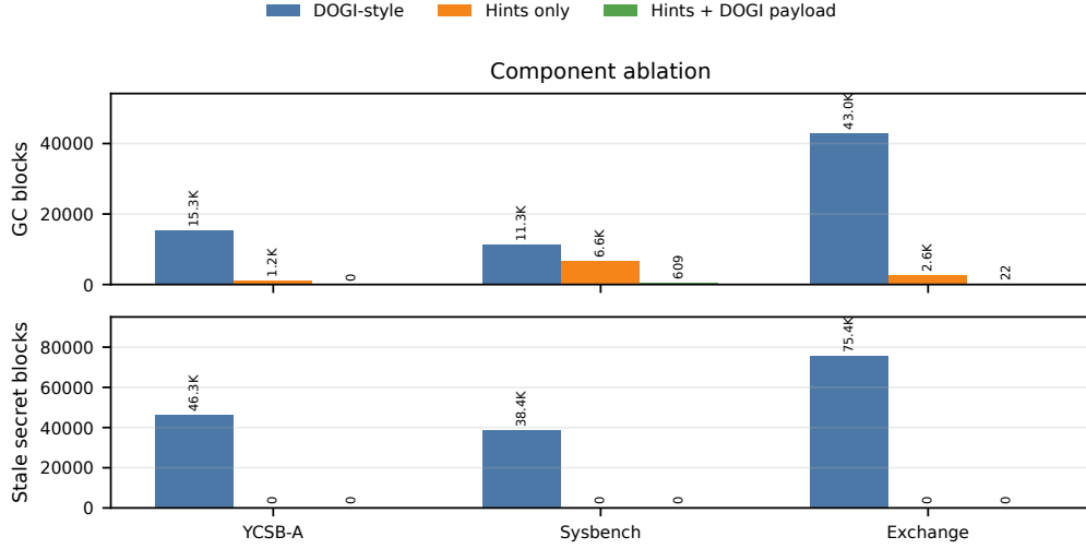
Figure 5: Component ablation. A history-only DOGI-style policy sees storage history but misses death cohorts, so GC and stale-secret exposure remain. Lifecycle hints remove exposure; adding DOGI-style payload fallback recovers payload placement and removes the remaining GC in the default hybrid.
