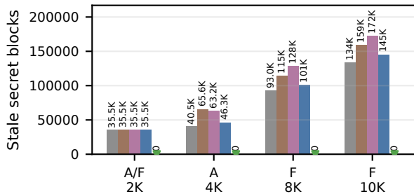
Expired-secret exposure
