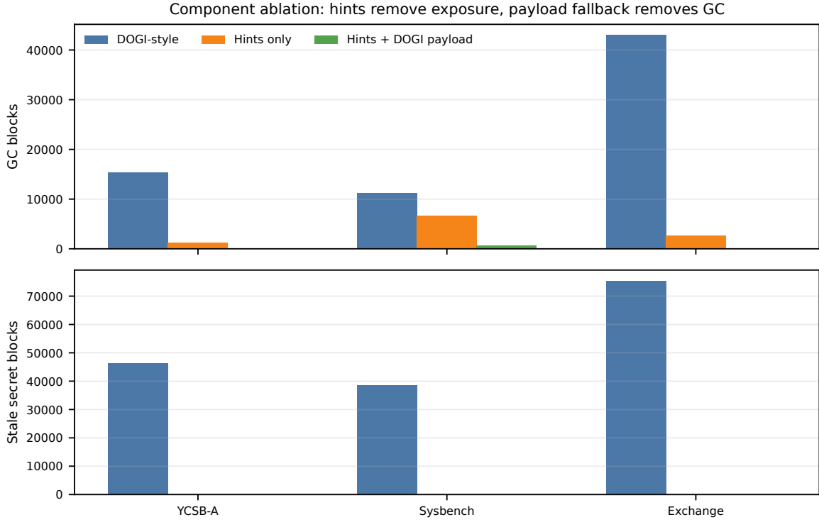
Figure 5: Component ablation. A history-only DOGI-style policy sees storage history but misses death cohorts, so GC and stale-secret exposure remain. Lifecycle hints remove exposure; adding DOGI-style payload fallback recovers payload placement and removes the remaining GC in the default hybrid.
