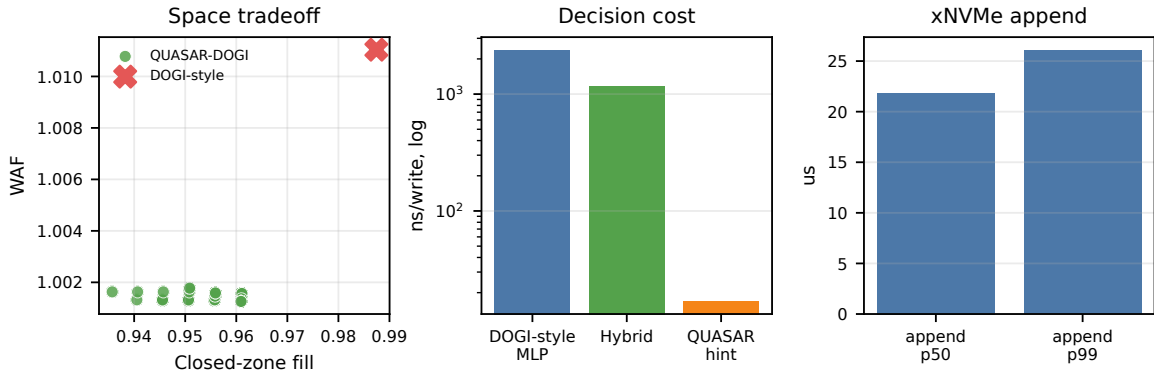
Figure 6: Resource and overhead controls. QUASAR-DOGI bounds the closed-zone fill cost while removing stale secrets, the hint-routing decision path is orders of magnitude cheaper than the DOGI-style policy-decision microbenchmark, and xNVMe confirms a lower-overhead append command path than the zonefs helper used for full-suite replay accounting.
