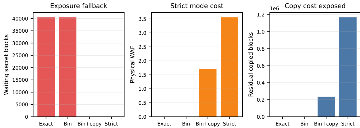
Figure 7: Robustness frontier. Exact and binned placement can leave straggler secrets waiting under tight active-zone budgets. Residual migration removes the exposure but increases physical WAF and copied blocks; strict zero-wait mode is therefore a policy point, not the default.
