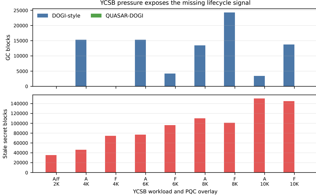
Figure 1: Actual-ZNS YCSB pressure. The low-pressure row is intentionally a negative WAF control, while higher PQC overlays create GC pressure. In both regimes, DOGI-style placement accumulates stale secret blocks because it cannot see protocol death cohorts; QUASAR-DOGI keeps secret cohorts reset-eligible and removes the exposure.
