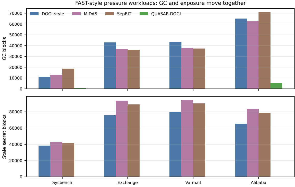
Figure 4: FAST-style pressure breadth. Sysbench, Exchange, Varmail, and Alibaba-like rows keep storage-visible locality while adding PQC lifecycle objects. History-based policies can still group payload, but they do not make expired secret cohorts reset-eligible; QUASAR-DOGI cuts GC and stale-secret exposure on the same pressure axes.
