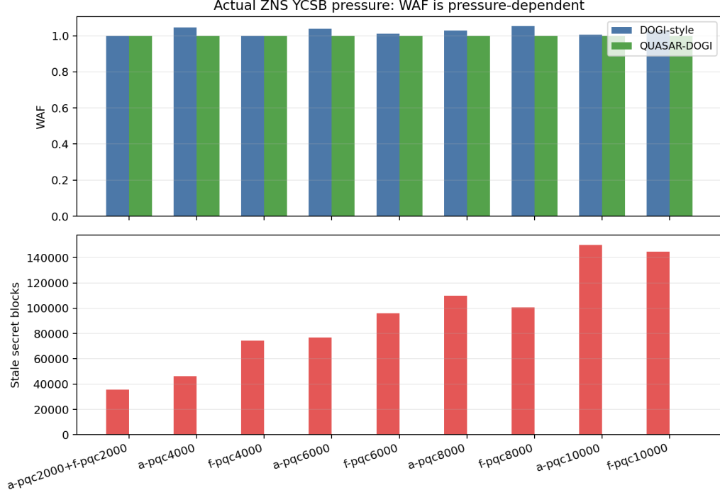
Figure 5: YCSB pressure curve on actual ZNS. The p2000 row is a negative control; p4000 through p10000 show where pressure creates GC/WAF separation. Across all rows, the stale-secret gap remains visible.
