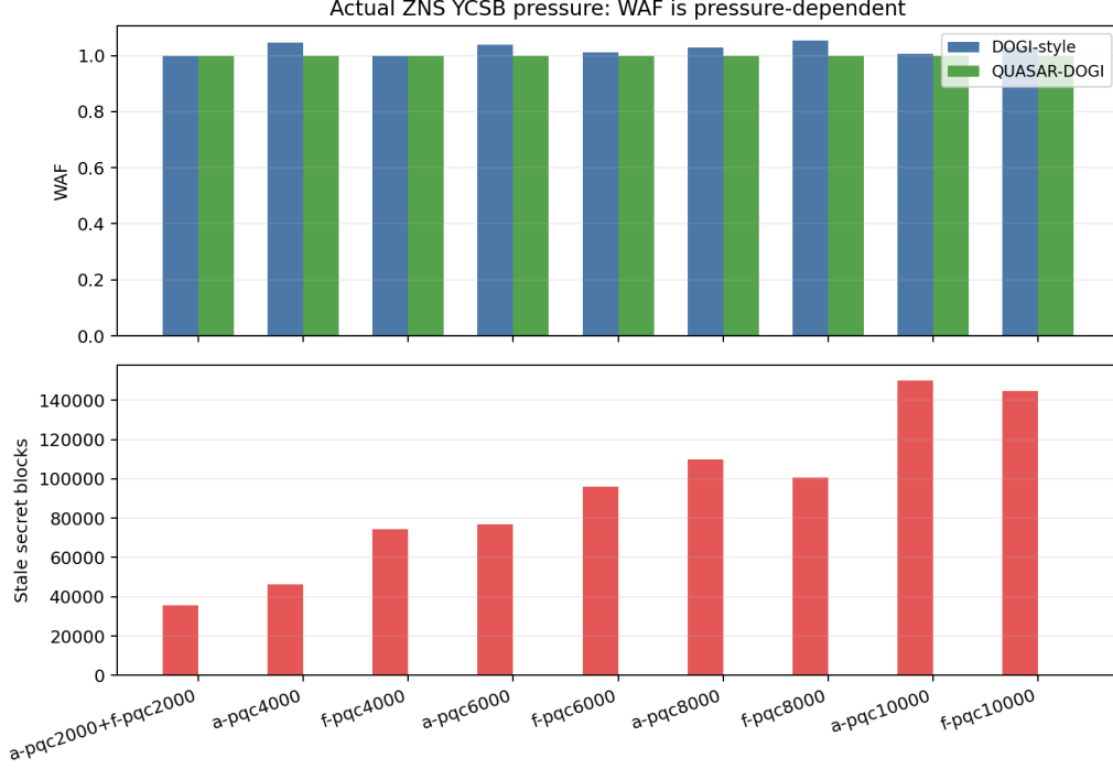
Figure 1: Actual-ZNS YCSB pressure curve. The low-pressure row is intentionally a negative WAF control: WAF is near 1.0 for history-based and hybrid policies, but expired secrets remain in non-resettable baseline zones. Higher PQC ratios create GC/WAF pressure while preserving the same semantic gap.
