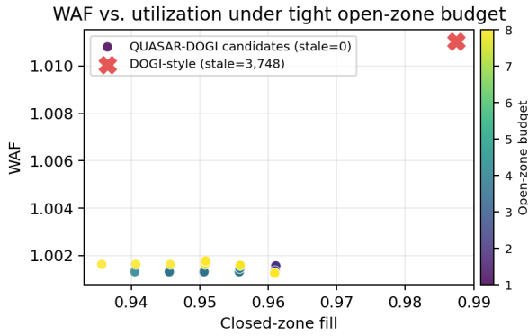
Figure 6: WAF vs. utilization sensitivity on Exchange p2000. QUASAR-DOGI candidates keep stale secrets at zero with closed-zone fill 0.936–0.961, while the DOGI-style point keeps higher fill but leaves 3,748 stale secret blocks.
