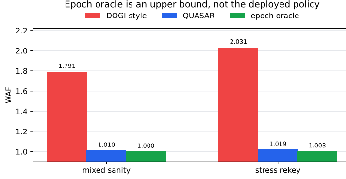
The gap shows that protocol lifetime is the missing placement signal; QUASAR uses lifecycle hints, not exact future delete timestamps.
