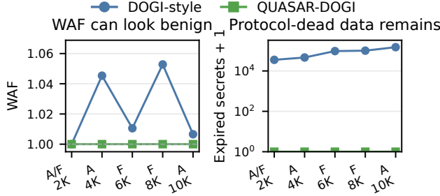
Figure 2: Motivation diagnostic: WAF is not enough to expose the PQC failure mode. DOGI-style placement can look benign on storage-visible WAF while still stranding expired PQC secrets; QUASAR-DOGI keeps payload on history placement but routes lifecycle objects by death cohort.
