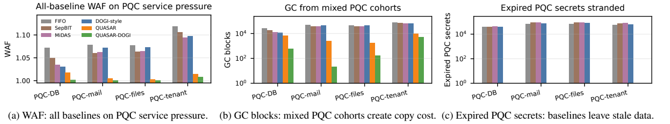
Figure 4: PQC lifecycle pressure breadth, comparing all same-path baselines. The x-axis names the service carrier, but the measured failure is PQC-specific: expired secret cohorts remain mixed with live payload under history-based placement. QUASAR and QUASAR-DOGI keep those cohorts reset-eligible while preserving payload placement on the history fallback.
