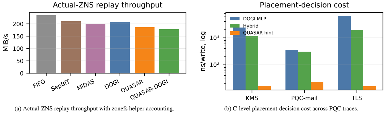
Figure 7: Prototype overhead in the role of DOGI's prototype figure. Full-suite actual-ZNS replay includes zonefs helper overhead and semantic reset commands, so it is an accounting bound rather than an optimized SPDK datapoint. The isolated C-level decision benchmark shows that lifecycle-hint routing is much cheaper than DOGI-style feature extraction and MLP scoring, while the hybrid keeps the DOGI fallback only where payload history is useful.
