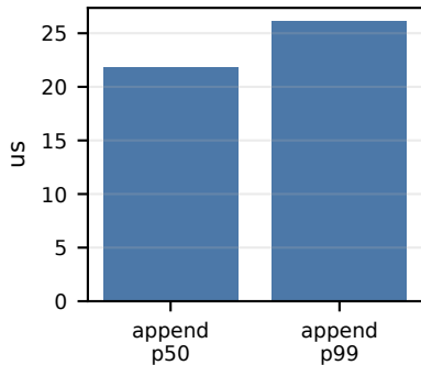
xNVMe append
