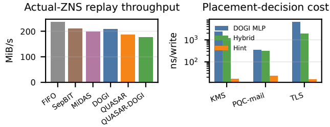
Figure 9: Prototype overhead in the role of DOGI's prototype figure. Zonefs replay is an accounting bound, while the isolated C-level benchmark shows lifecycle-hint routing is much cheaper than DOGI-style feature extraction and MLP scoring.
