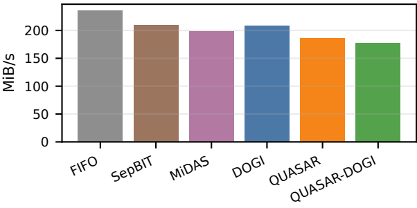
Actual-ZNS replay throughput
