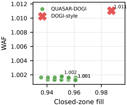
PQC placement space cost
