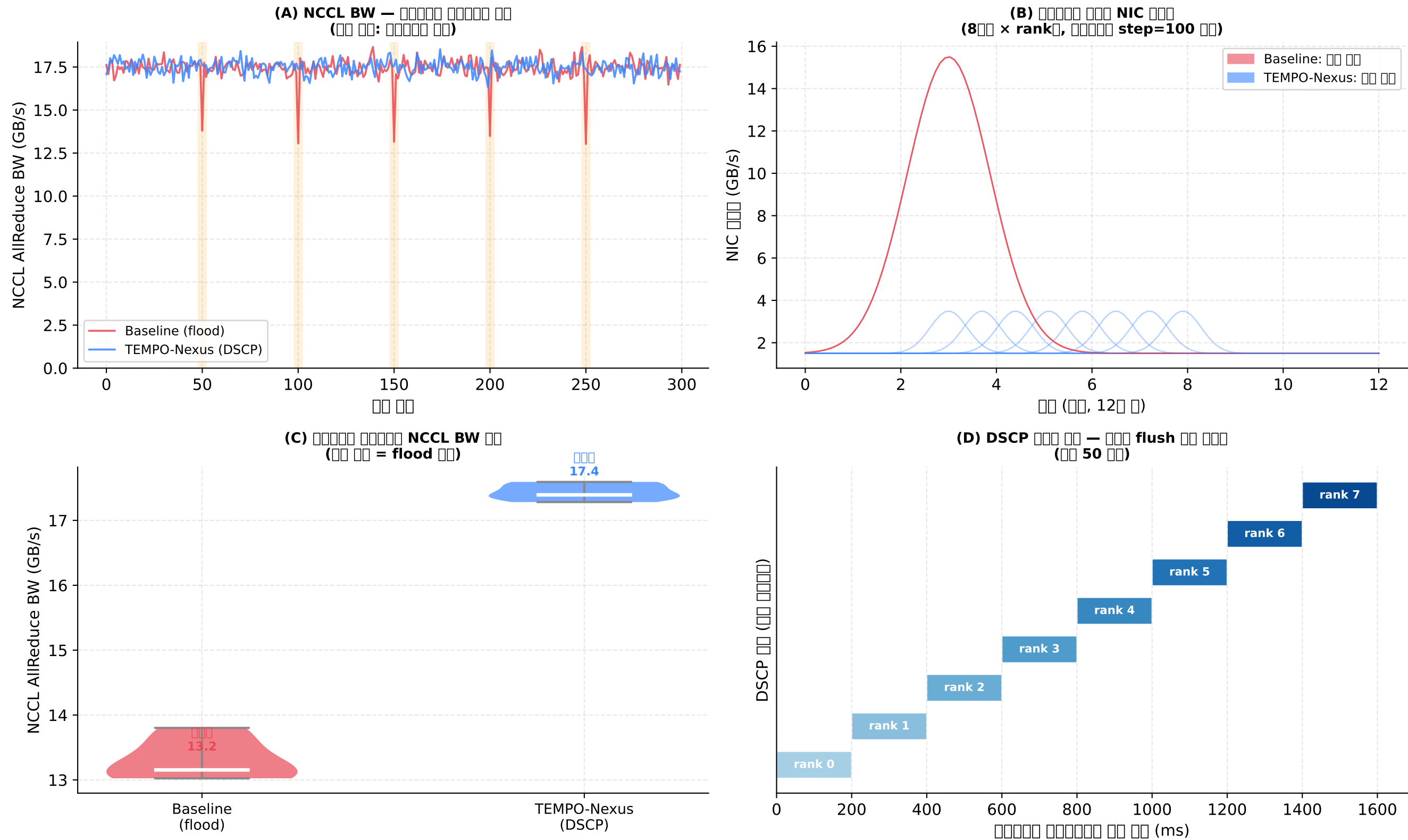
Fig 12. TEMPO-Nexus: 8-rank flush → Slingshot
