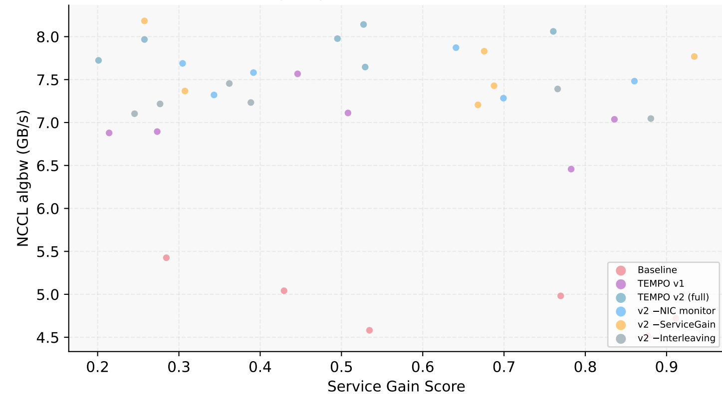
Service Gain vs. NCCL BW at Ckpt Steps (higher gain → bandwidth preserved)
