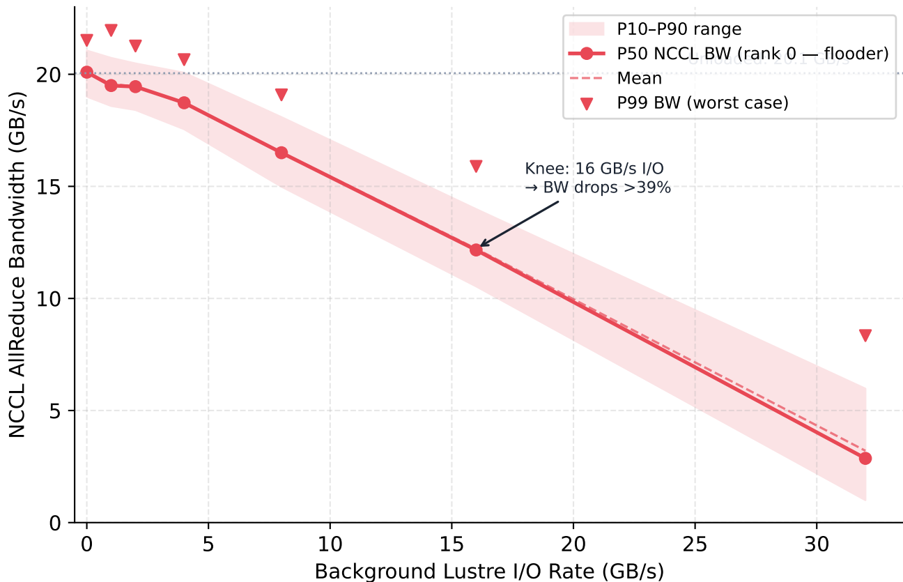
Fig 10 — Slingshot-11 Fabric Sharing: Lustre I/O Degrades NCCL Bandwidth (Perlmutter, 2 nodes × 4×A100, AllReduce 256 MB)
