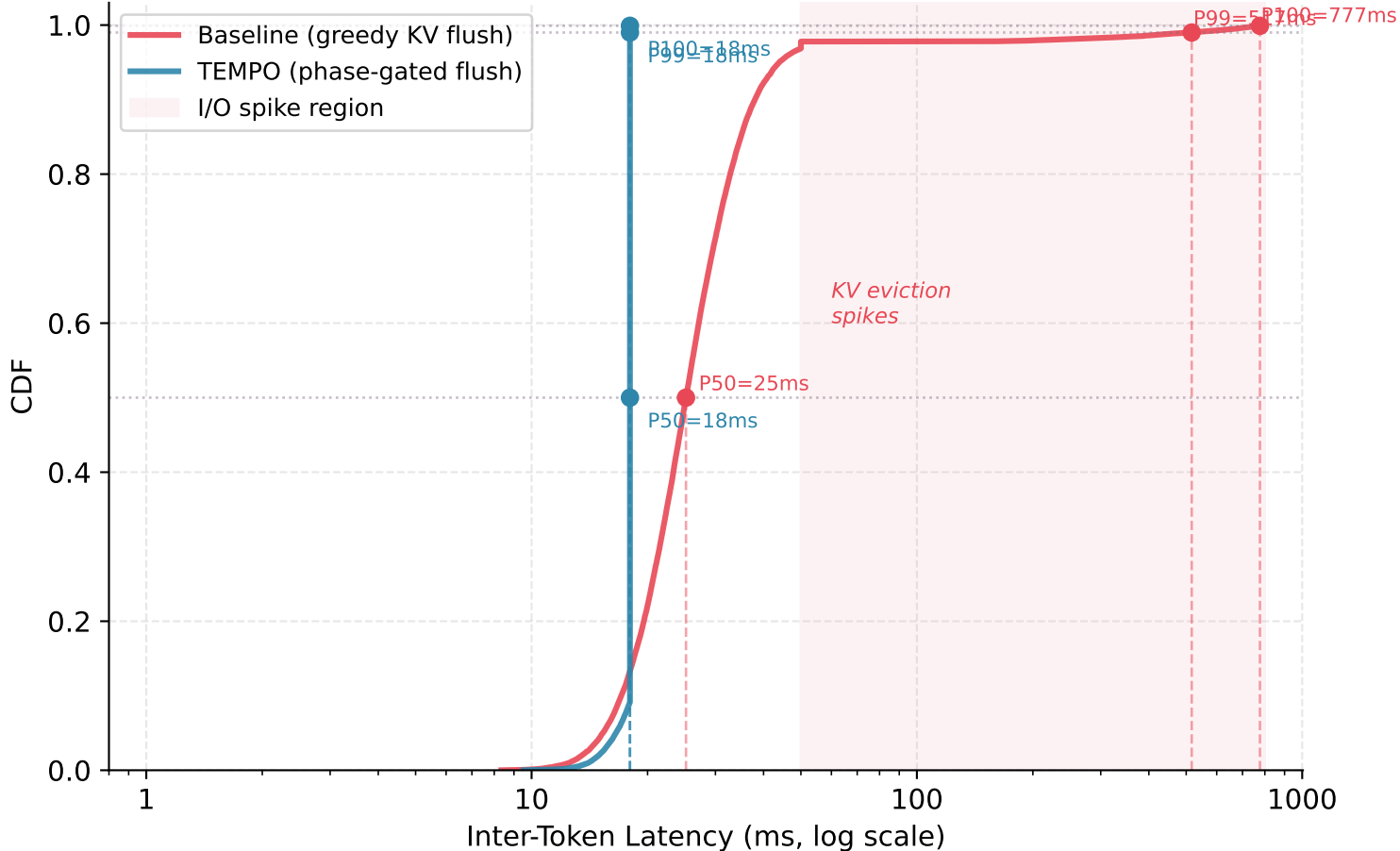
Fig 11 — ITL Tail Latency CDF under BurstGPT Traffic (vLLM, Llama-2-7B, tensor_parallel=4, gpu_util=0.65)
