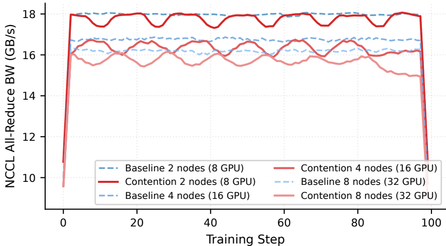
PCIe Contention Scales With Node Count
