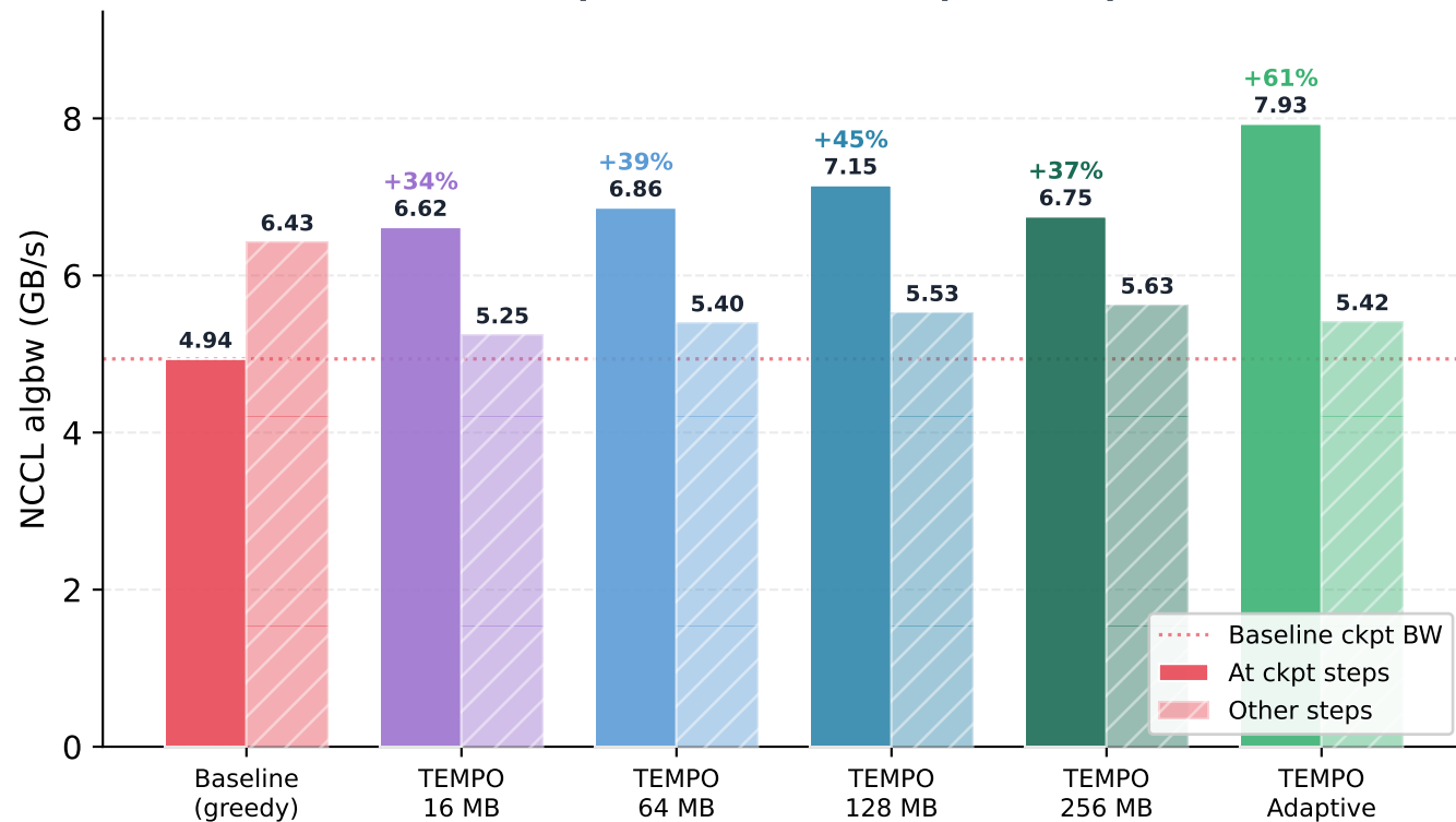
NCCL BW by Chunk Size at Checkpoint vs. Non-Checkpoint Steps
