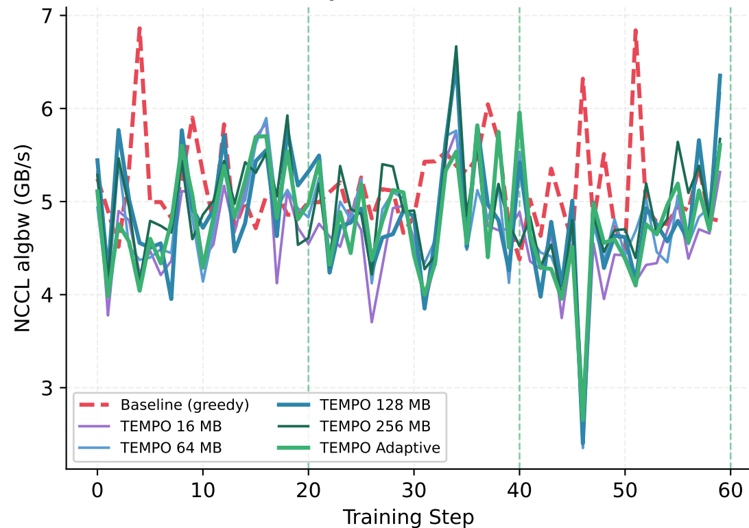
Per-Step BW: All Chunk Sizes
