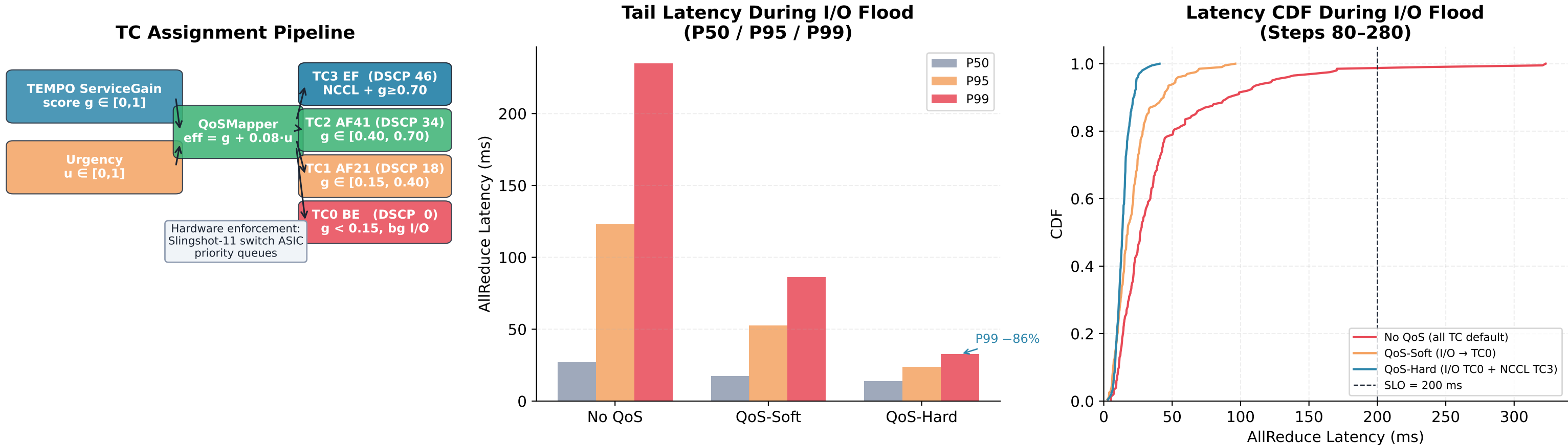
Fig 10: TEMPO v3 Slingshot-11 Hardware QoS — Service-Gain → Traffic-Class Mapping (2N×4×A100, Perlmutter Slingshot-11, simulated)
