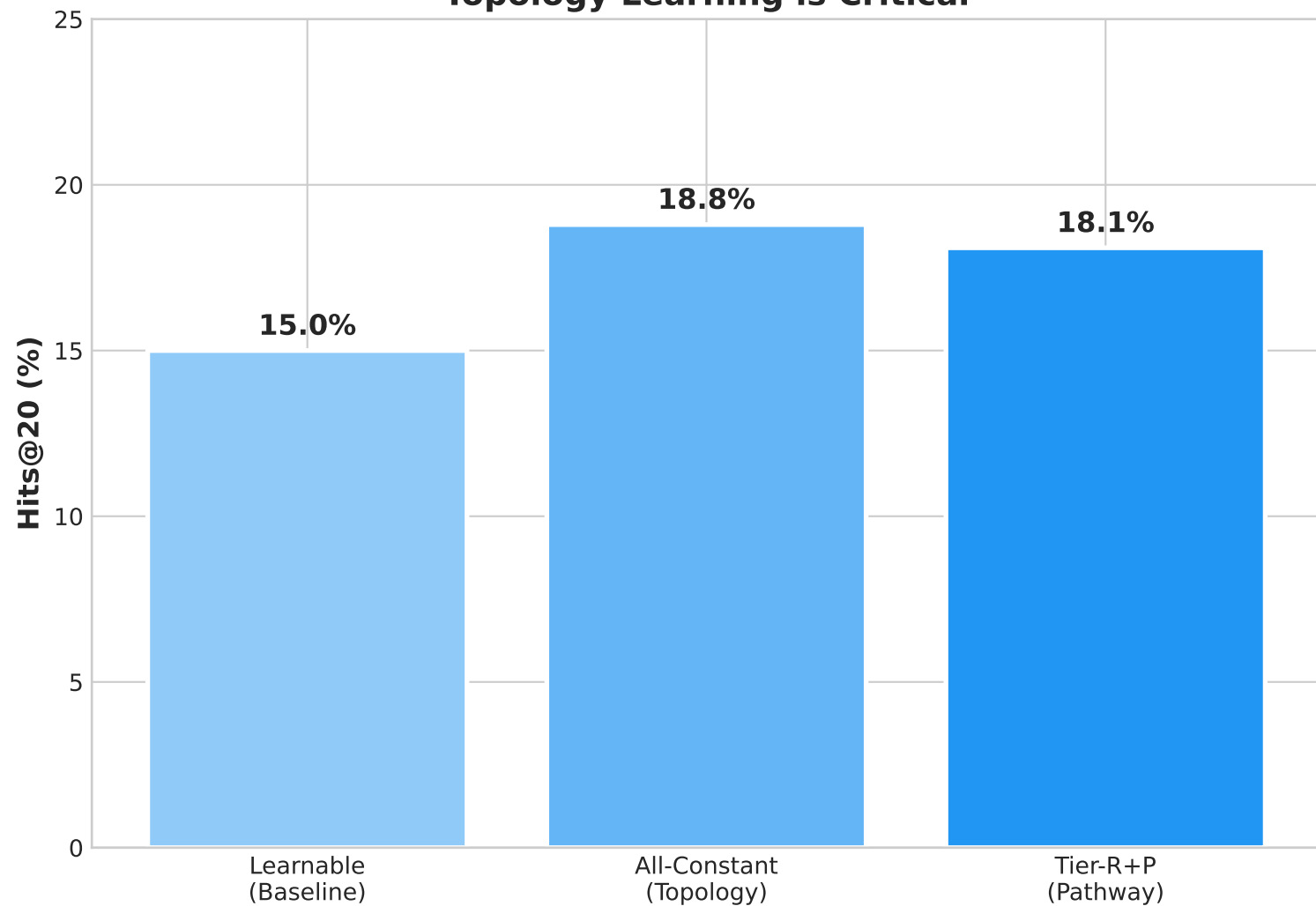
Figure S3: Track A - Ablation Study Topology Learning is Critical
