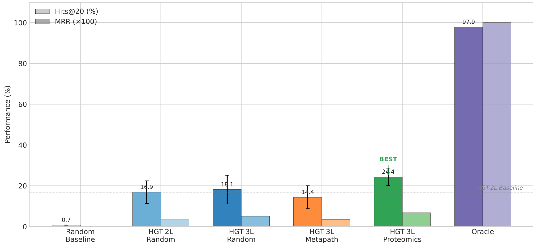
GNN Model Performance Comparison
