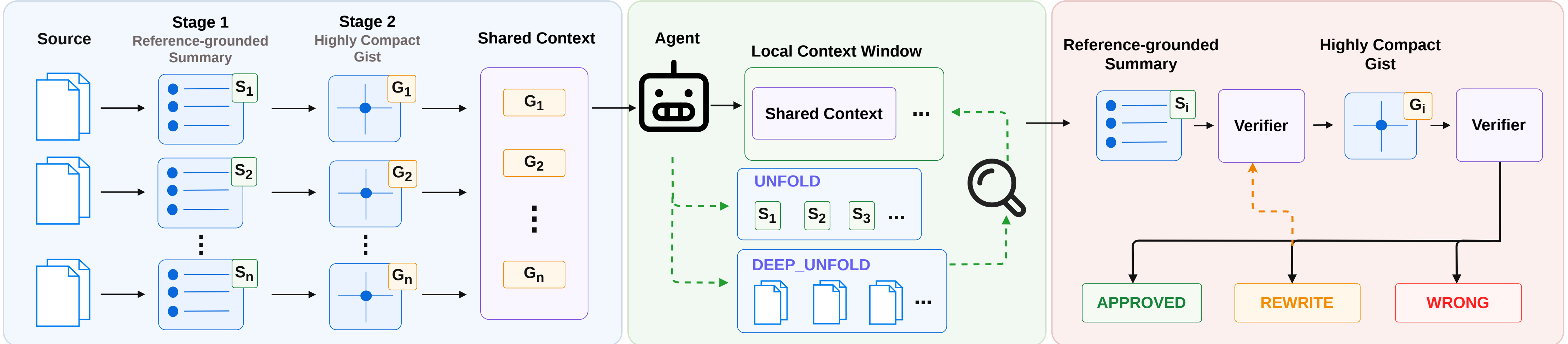
(a) Shared Context + Summarization
