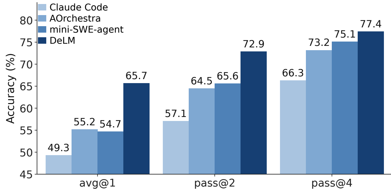
SWE-bench Verified (Base: Gemini-3-Flash)
