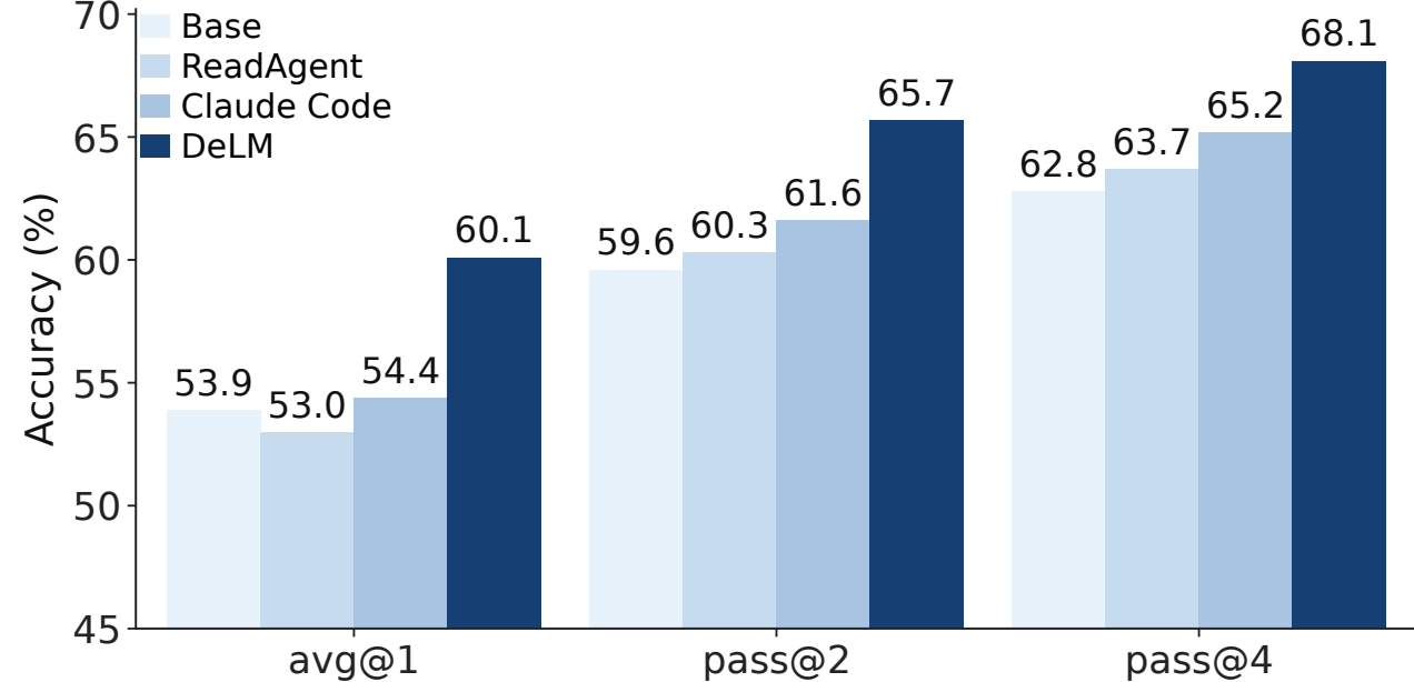
LongBench-v2 Multi-Doc QA (Base: GPT-5.4)
