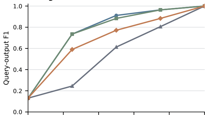
a Flights
