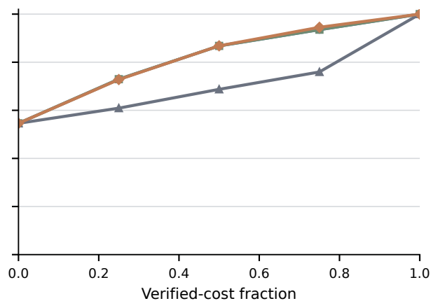
d Beers
