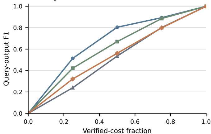
c Hospital
