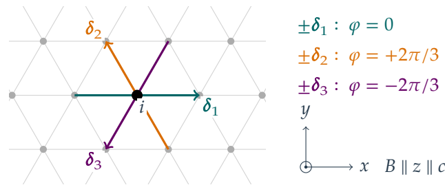
Figure 2. Triangular lattice and nearest-neighbor vectors \delta_{1,2,3} . Opposite bonds share the indicated phase; \delta_1 \parallel x . The dot-in-circle denotes a field out of the plane.
