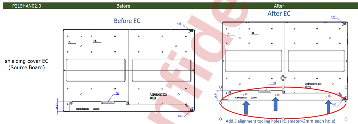
Figure : Add 3 tooling alignment holes (P215HAN02.0).png
