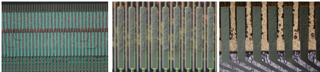
Conductive particle(IC Bonding) normal
