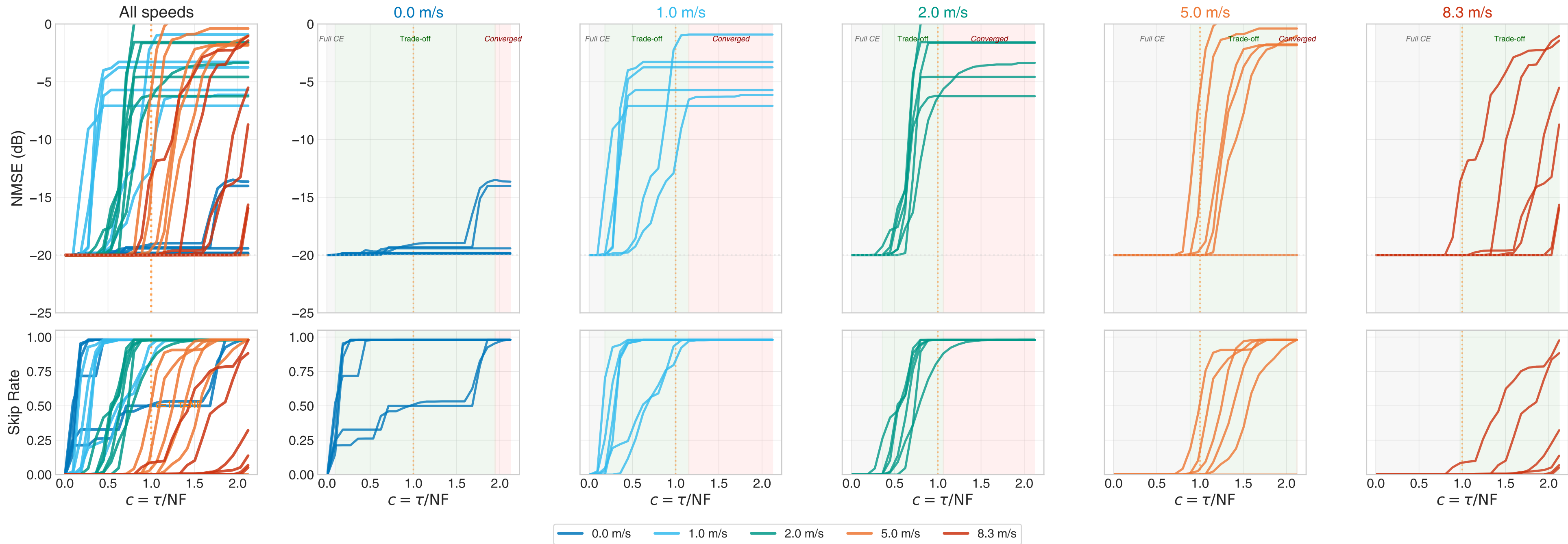
Fig 3: CE Skip Threshold Analysis ( \delta_{oracle} , binary) — ELAA 28GHz
