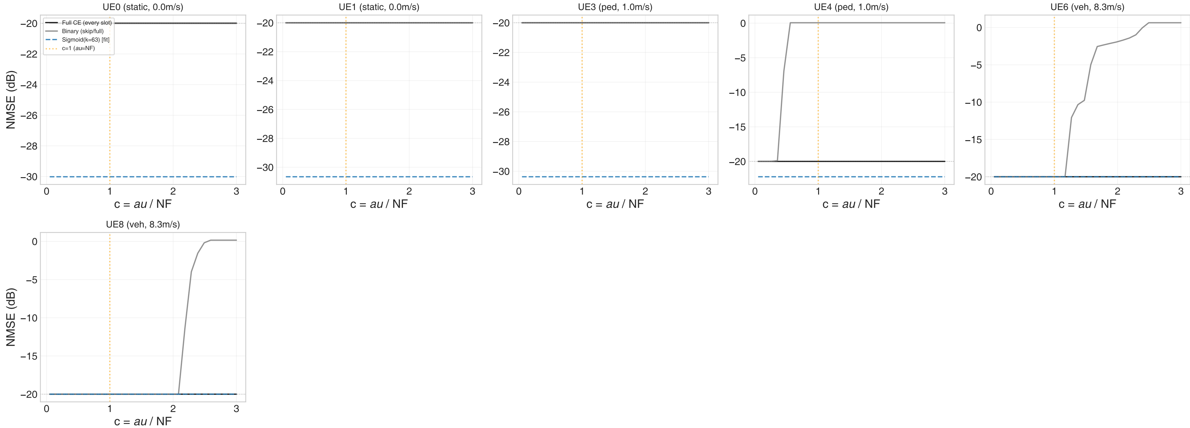
Fig 3b: \alpha Scheduling Strategies (ELAA 15GHz, Oracle \delta , 200 slots) c=1.0 is the safe operating point ( \tau = noise floor)
