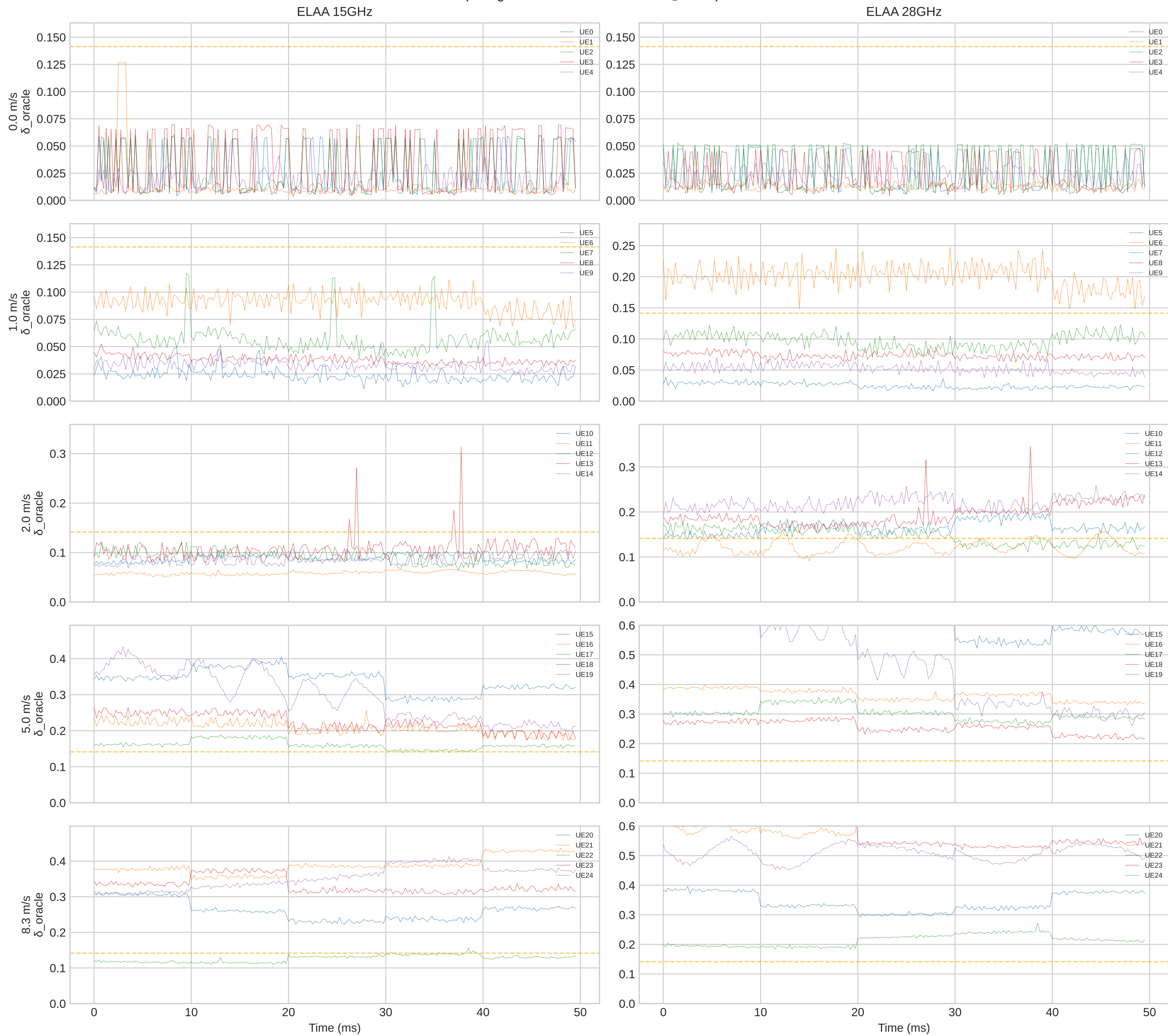
Fig 2: Oracle Channel Variation \delta(t) across Configs and Mobility (orange dashed = LS noise floor @20dB)
