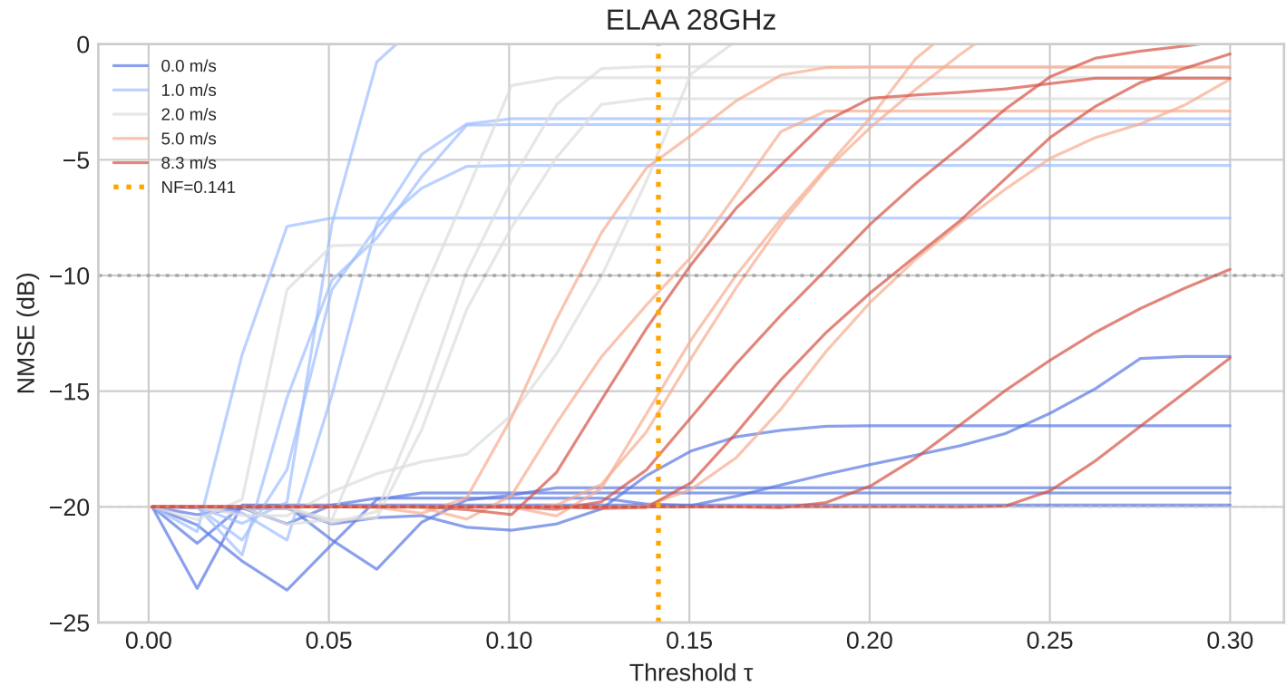
Fig 3: NMSE vs Skip Threshold (Oracle \delta scheduling, EMA \alpha=0.7 )
