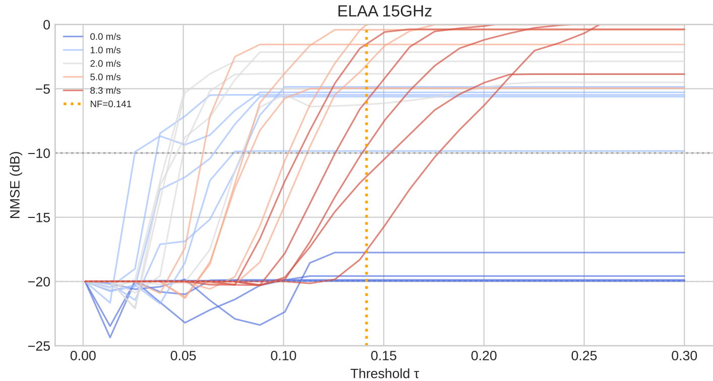
Fig 3: NMSE vs Skip Threshold (Oracle \delta scheduling, EMA \alpha=0.7 )
