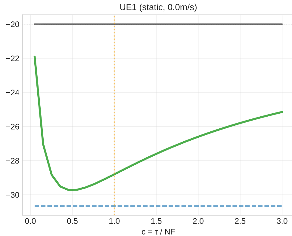
Fig 3b: \alpha Scheduling Strategies (ELAA 15GHz, Oracle \delta , 200 slots) c=1.0 is the safe operating point ( \tau = noise floor)
