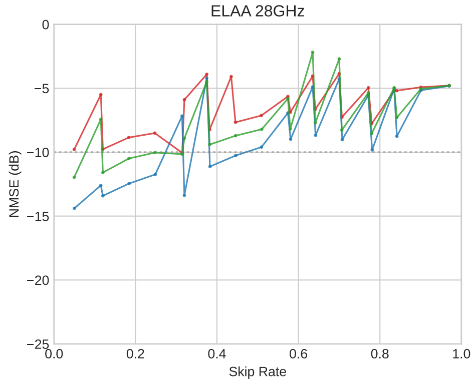
Fig 4: Feature Comparison — Skip Rate vs NMSE (EMA \alpha=0.7 )
