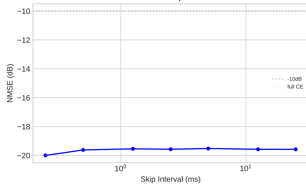
NMSE vs Skip Interval
