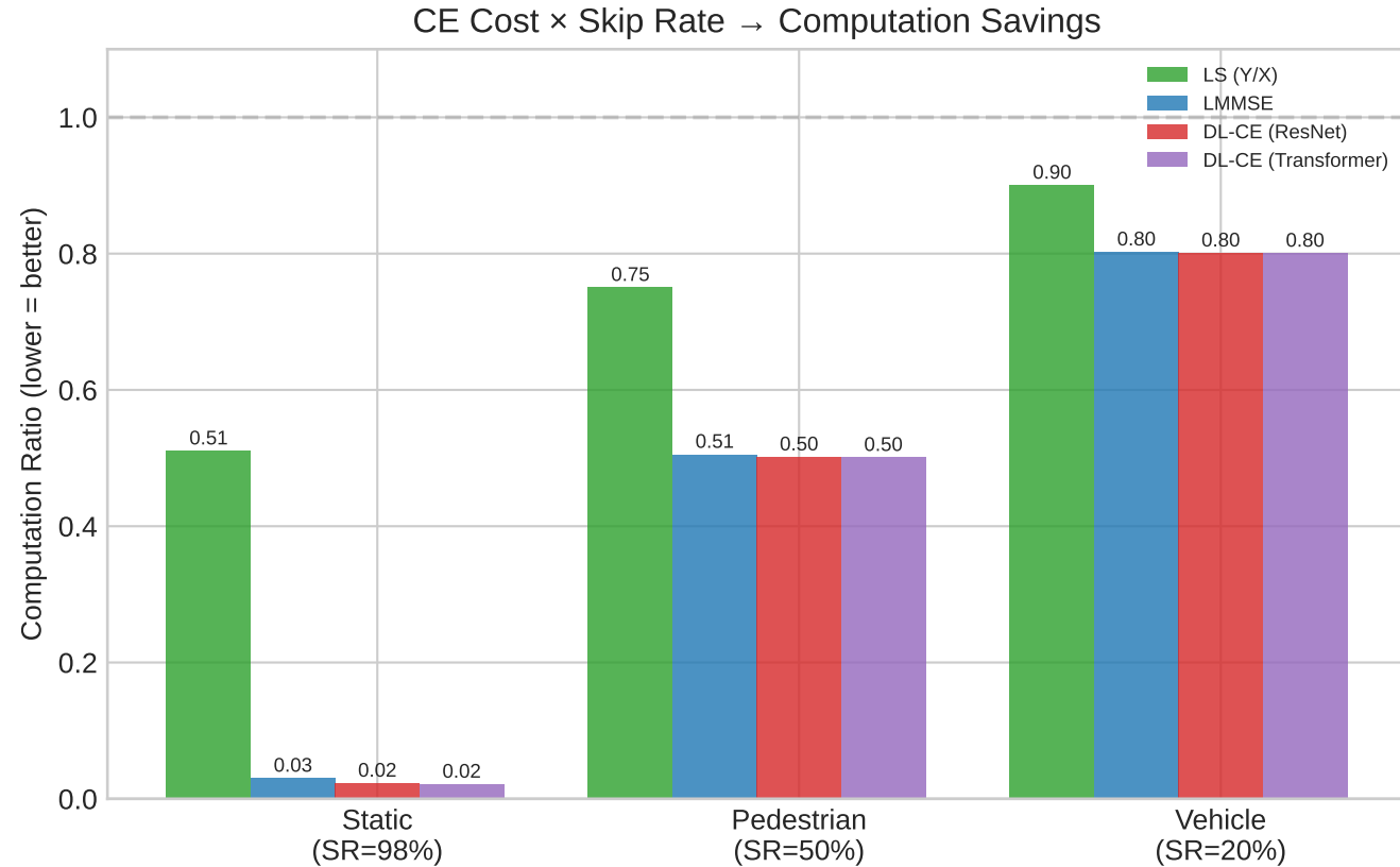
Fig 6: CE Skip Savings Scale with CE Complexity (NMSE tradeoff is CE-agnostic, but time savings are CE-specific)
