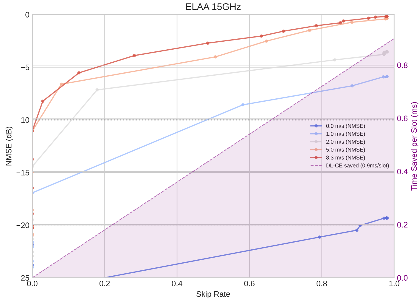
Fig 7: CE Skip Tradeoff — NMSE vs Computation Savings (LS scheduling @20dB, EMA \alpha=0.7 , Small PACENet 0.9ms)
