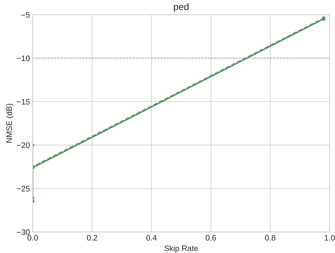
Fig 8: DL-CE Model Size \times Skip Tradeoff (ELAA 15GHz)
