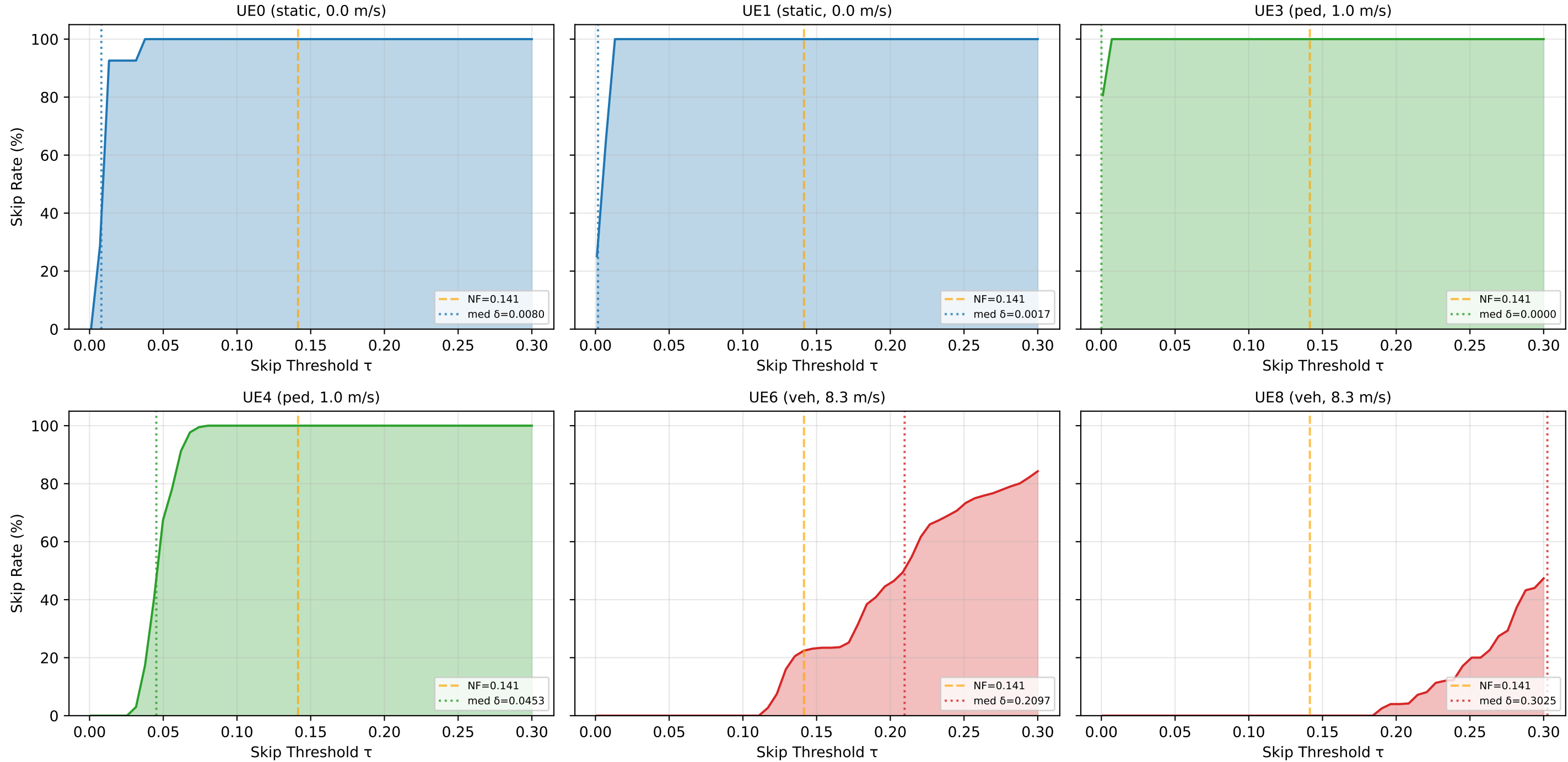
Skip Rate vs Threshold \tau per UE (Oracle \delta , ELAA 15GHz) Higher = more slots skipped = more computation saved
