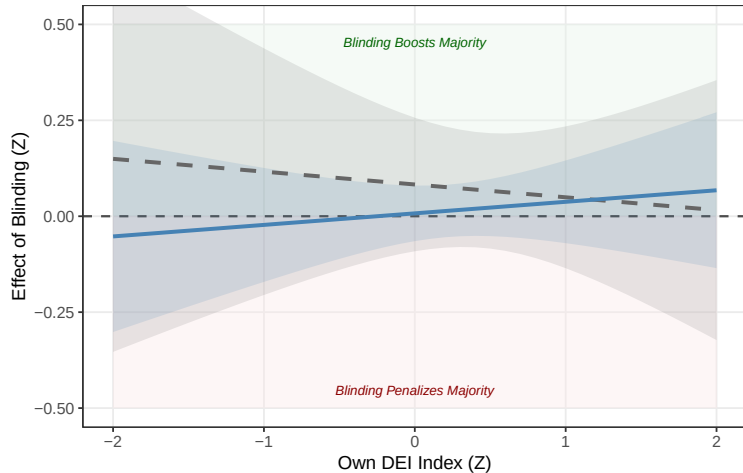
HR --- Majority
