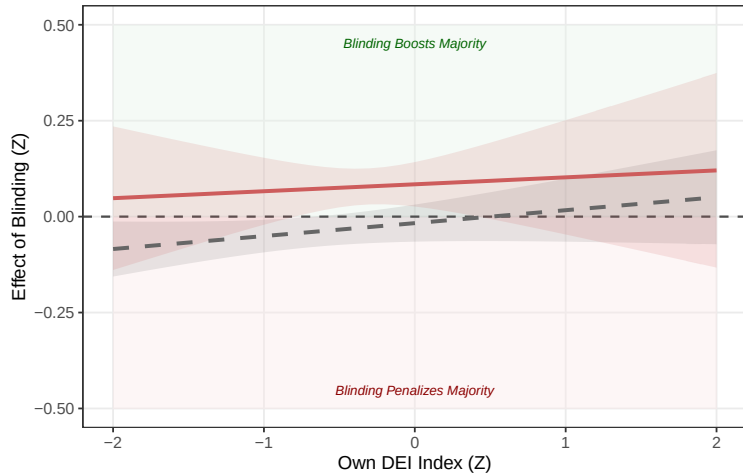
Eng --- Majority
