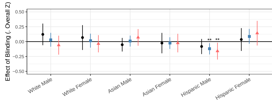
HR: URM-axis, by GPA
