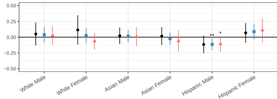
HR: URM-axis, by Coding
