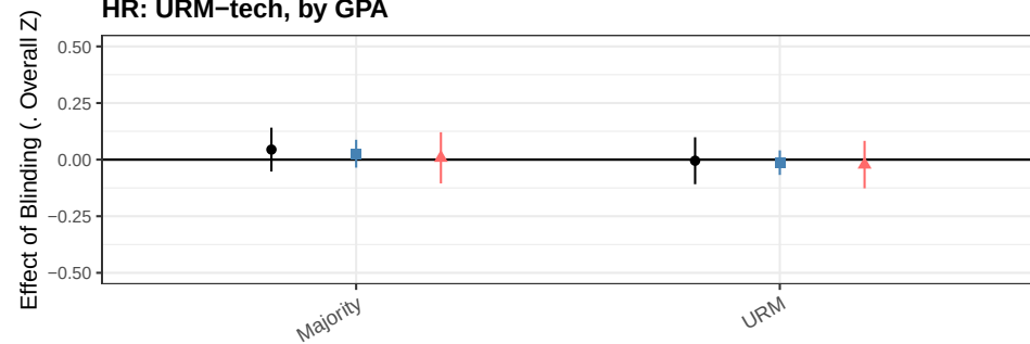
HR: URM-tech, by GPA
