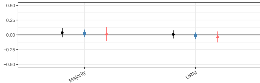
HR: URM-tech, by Coding
