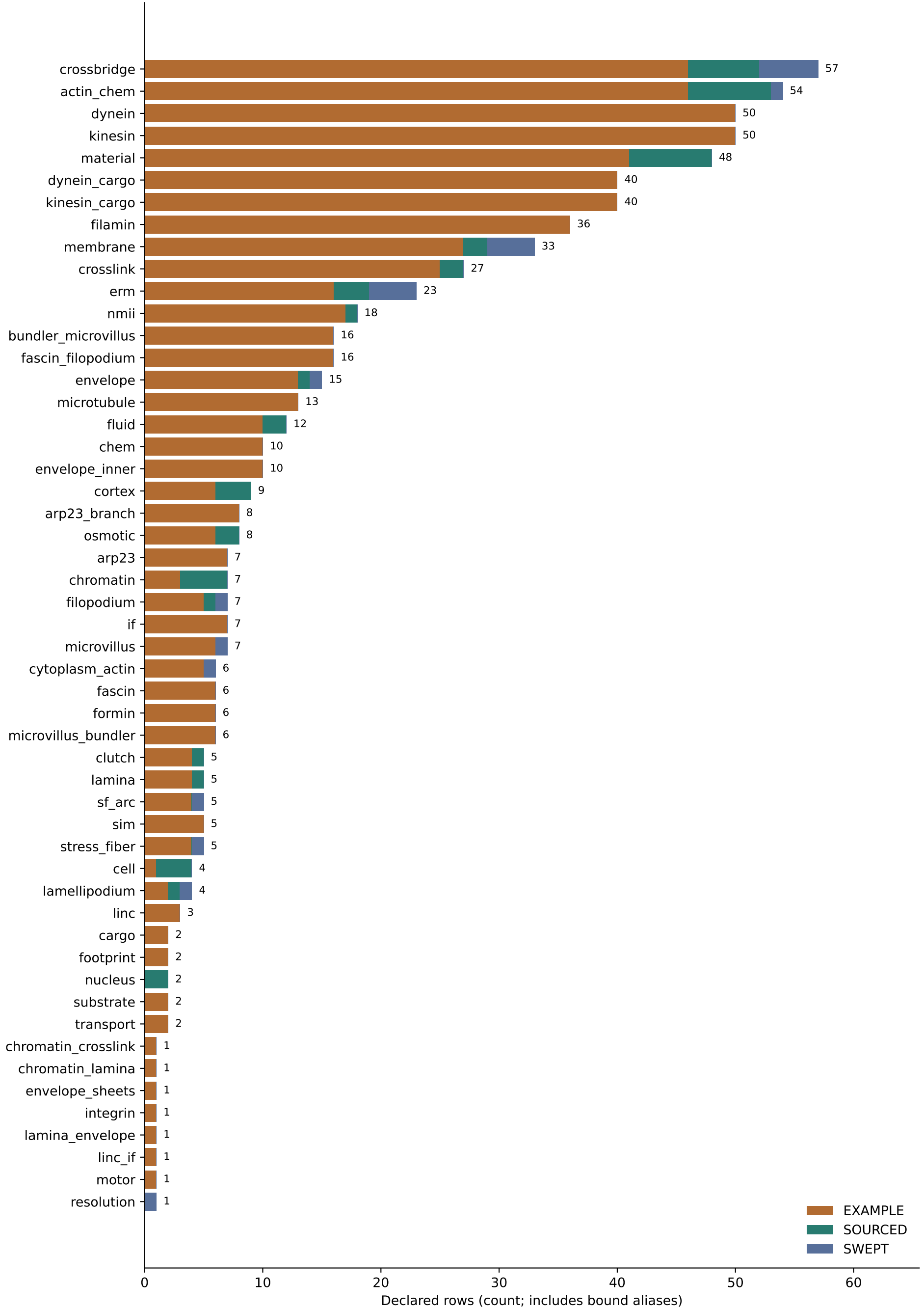
Parameter declarations by group 706 rows = 565 valued inputs + 141 aliases
